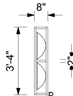
SIDE VIEW
